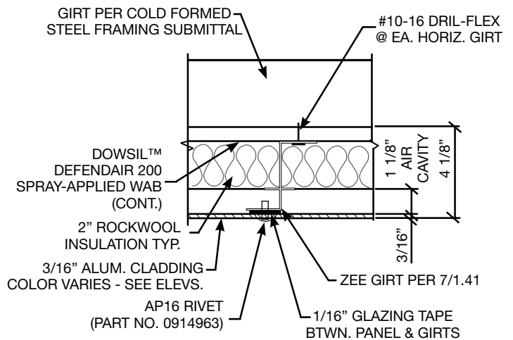
1 TYPICAL ASSEMBLY SCALE: 3" = 1'-0"
