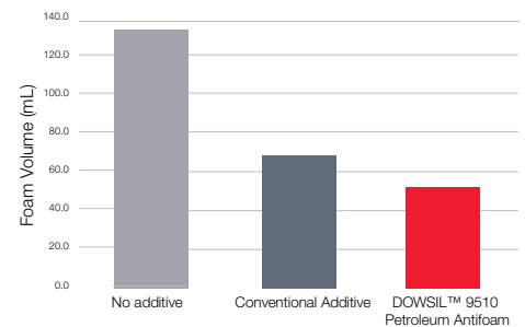
Figure 1 – Initial foam volume in 80 mL of crude API 26°
