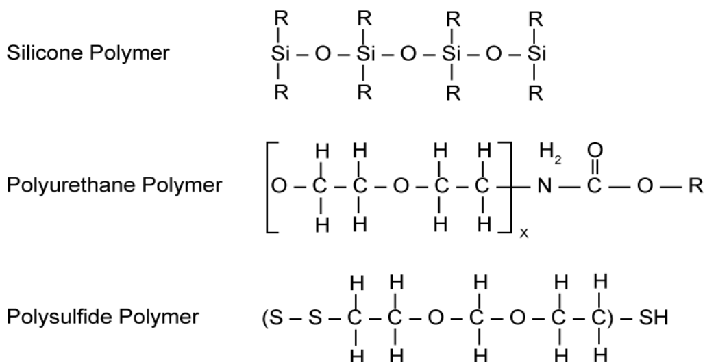
Figure 1: Sealant Polymer Formulations
