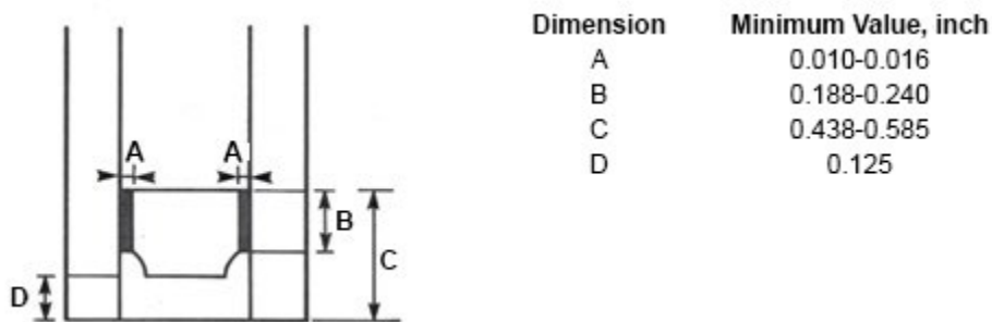
Figure 11: SIGMA Survey Recommended Seal Dimensions for Conventional (Dry Glazed) Dual Seal Unit, Silicone Secondary Seal 22
