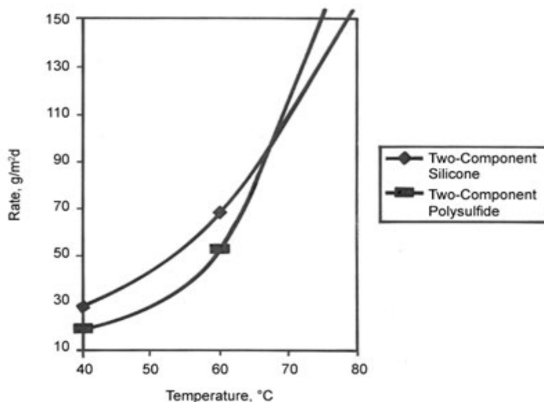
Figure 5: Silicone and Polysulfide Water Vapor Permeability for a 3-mm Membrane 11
