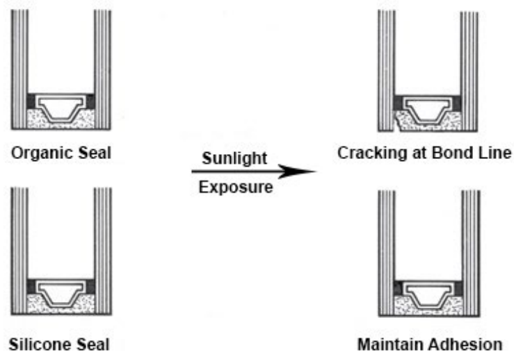
Figure 3: Sunlight Effect on Insulating Glass Unit Seals 8
