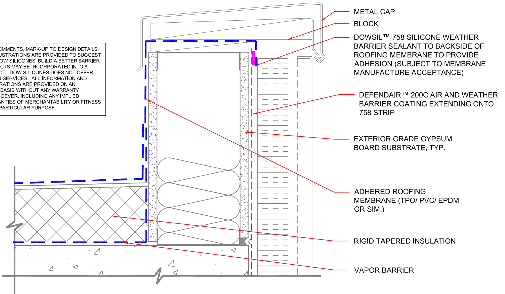
DETAIL SECTION: PARAPET ADHERED ROOFING INSTALLED AFTER DEFENDAIR™ 200C AIR AND WEATHER BARRIER COATING
