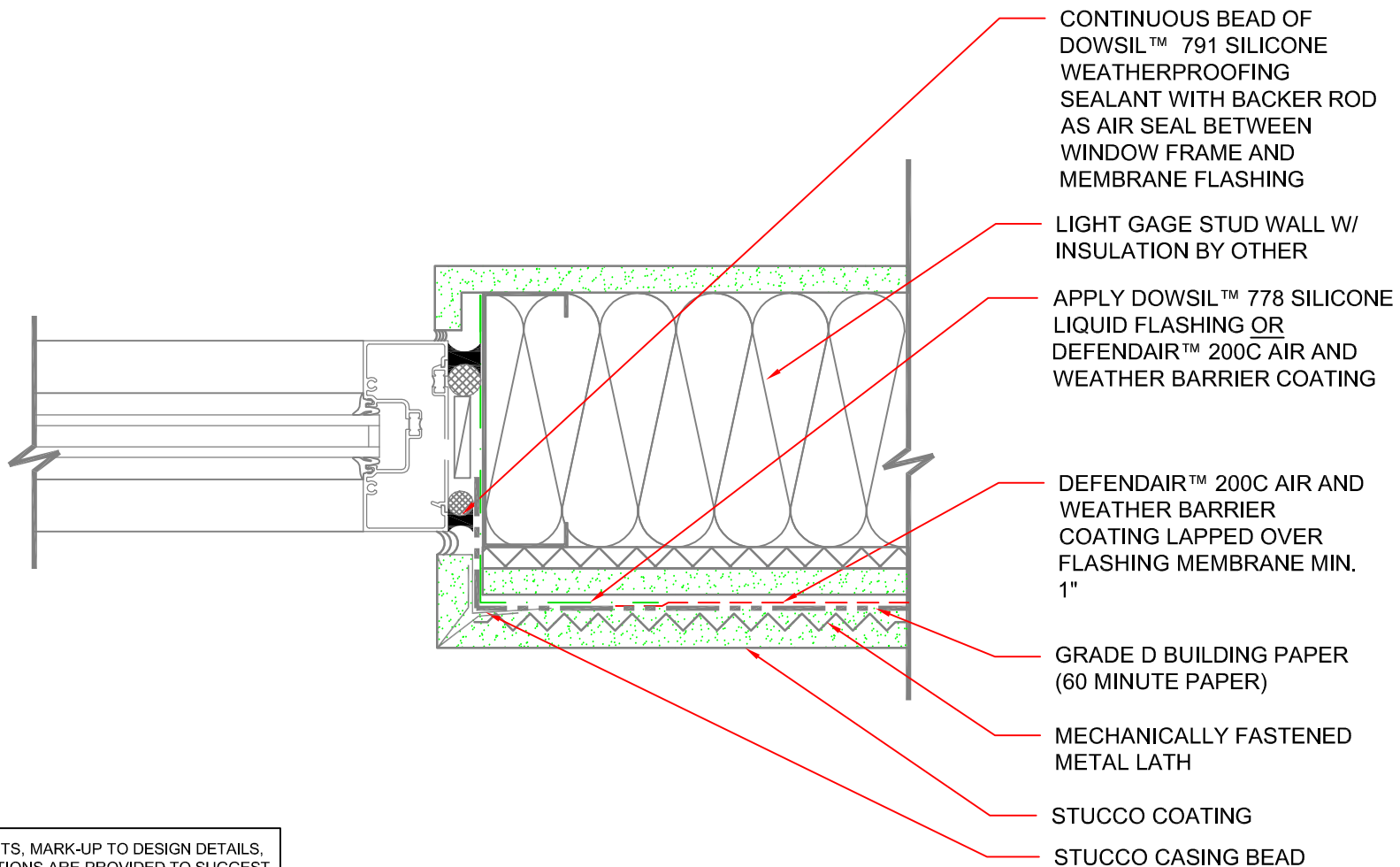
222 DETAIL SECTION: STOREFRONT JAMB AT STUCCO ON LIGHT GAGE STUD WALL SCALE: 3"=1'-0"
