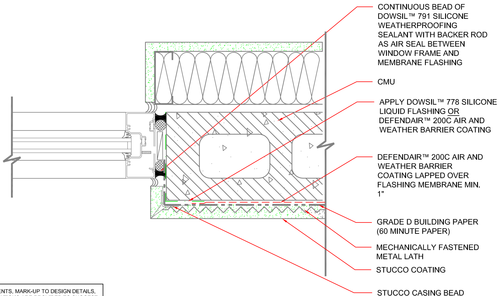
212 DETAIL PLAN: STOREFRONT JAMB AT STUCCO ON MASONRY WALL SCALE: 3"=1'-0"
