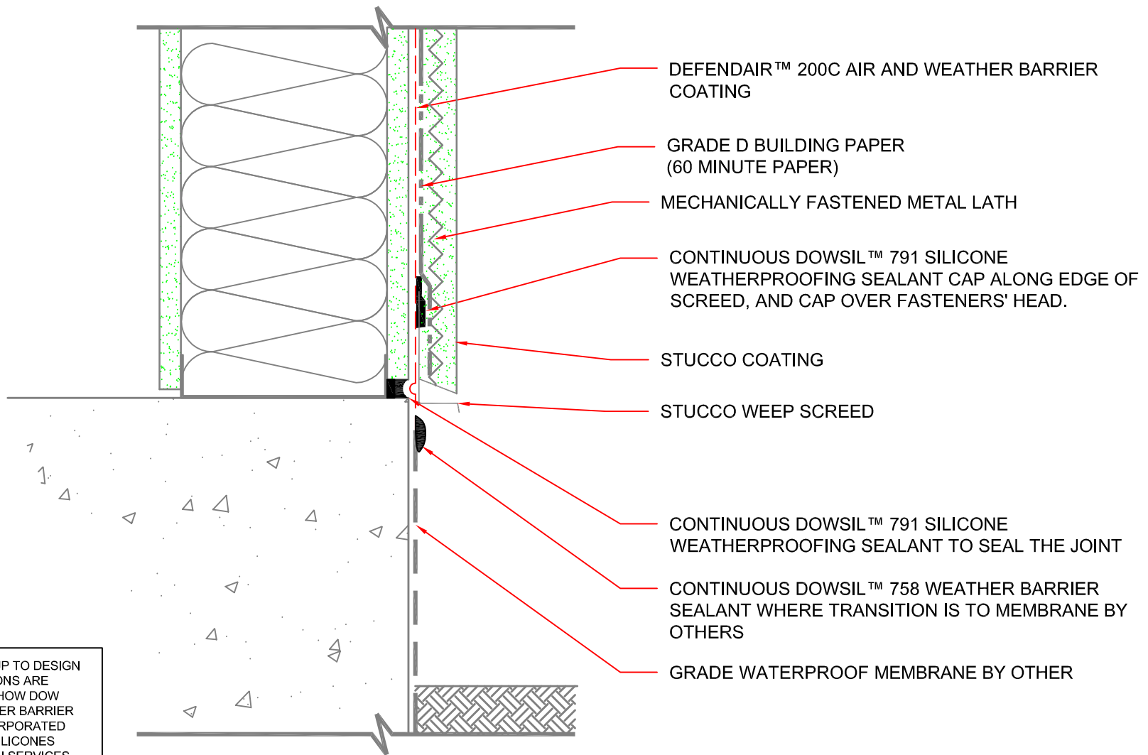
201a DETAIL SECTION: BASE WALL AT STUCCO ON LIGHT GAGE WALL SCALE: 3"=1'-0"
