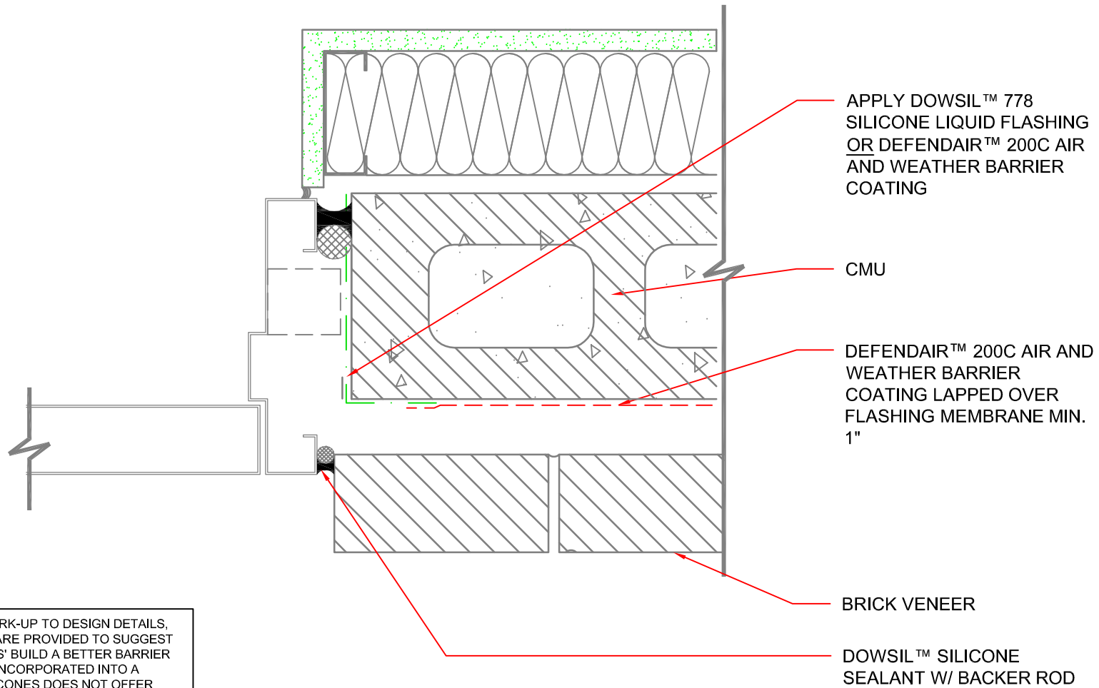
131 DETAIL PLAN: H.M. DOOR AT BRICK W/ CMU WALL SCALE: 3"=1'-0"
