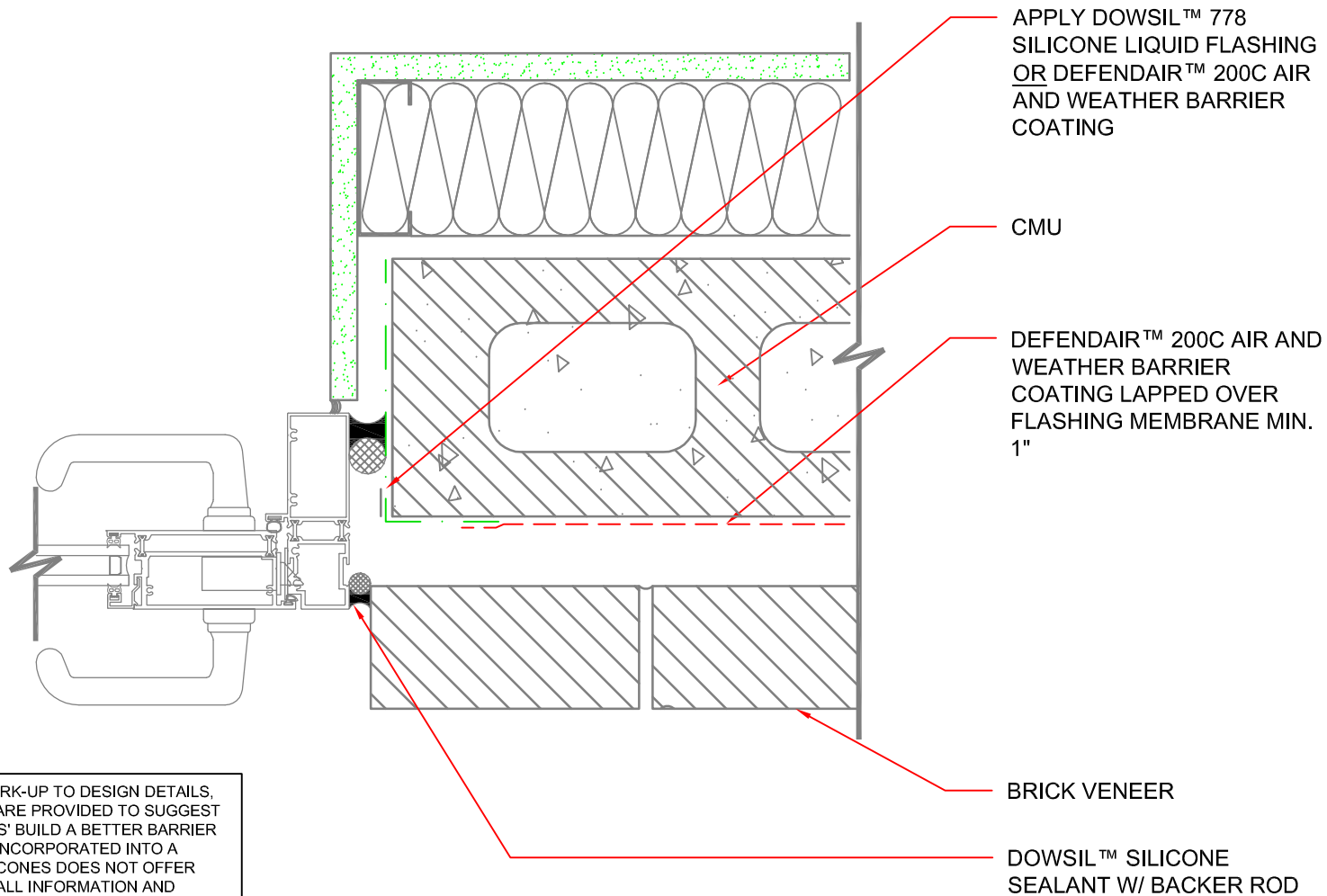
130 DETAIL PLAN: DOOR AT BRICK W/ CMU WALL SCALE: 3"=1'-0"
