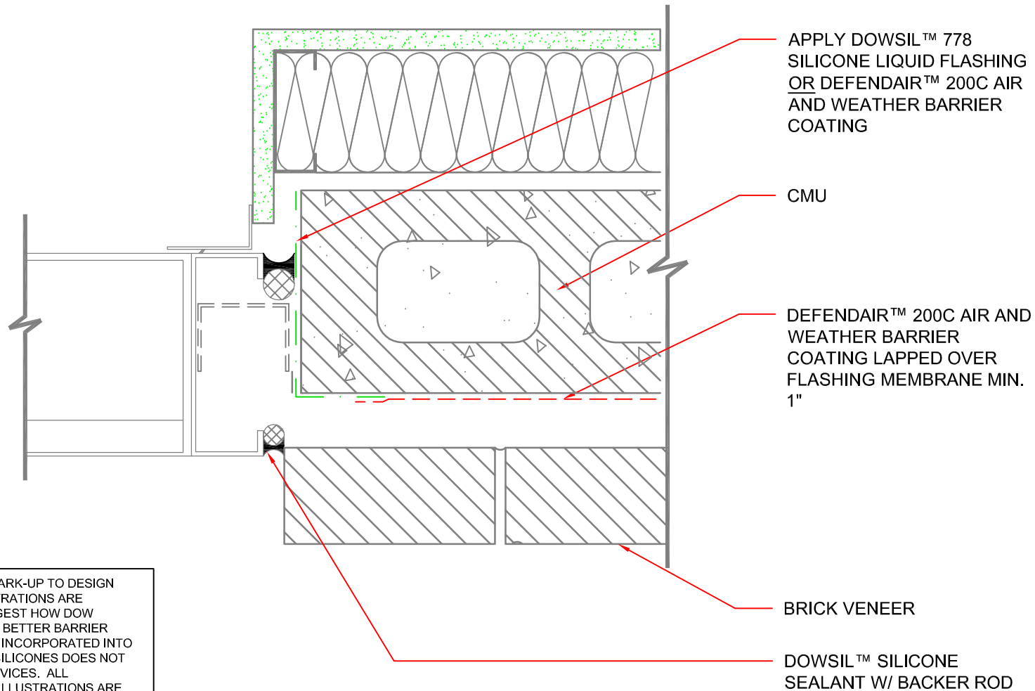
127 DETAIL PLAN: LOUVER AT BRICK W/ CMU WALL SCALE: 3"=1'-0"
