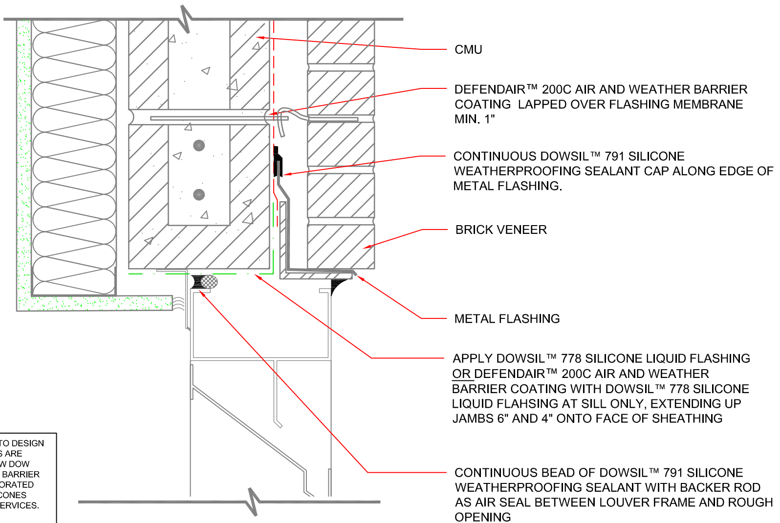
125 DETAIL SECTION: HEAD: LOUVER AT BRICK W/ CMU WALL SCALE: 3"=1'-0"
