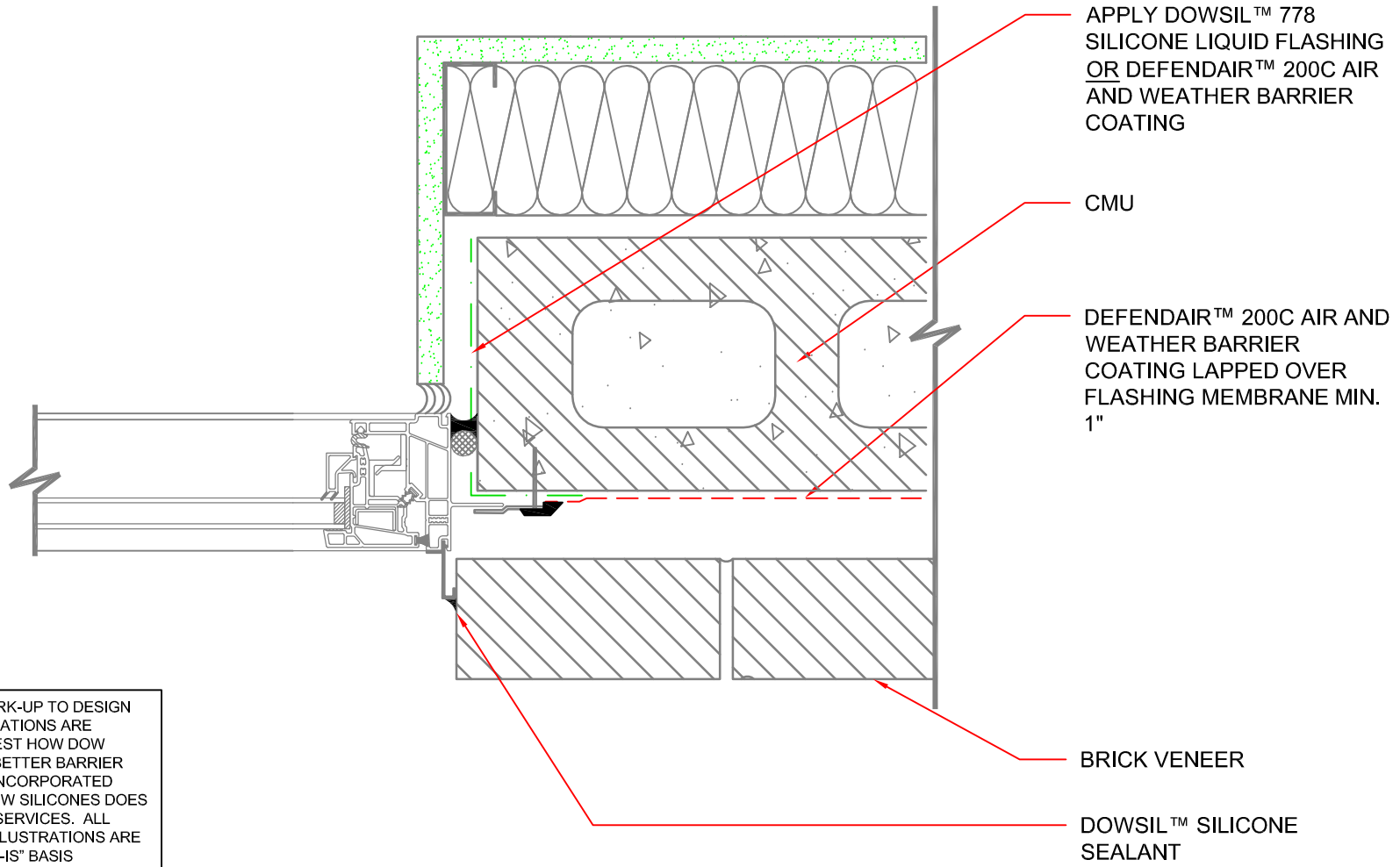
118 DETAIL PLAN: FLANGE WINDOW AT BRICK W/ CMU WALL SCALE: 3"=1'-0"
