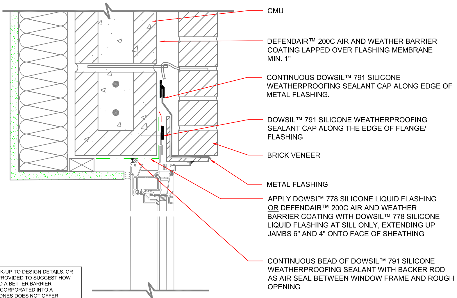
116 DETAIL SECTION: HEAD: FLANGE WINDOW AT BRICK W/ CMU WALL SCALE: 3"=1'-0"
