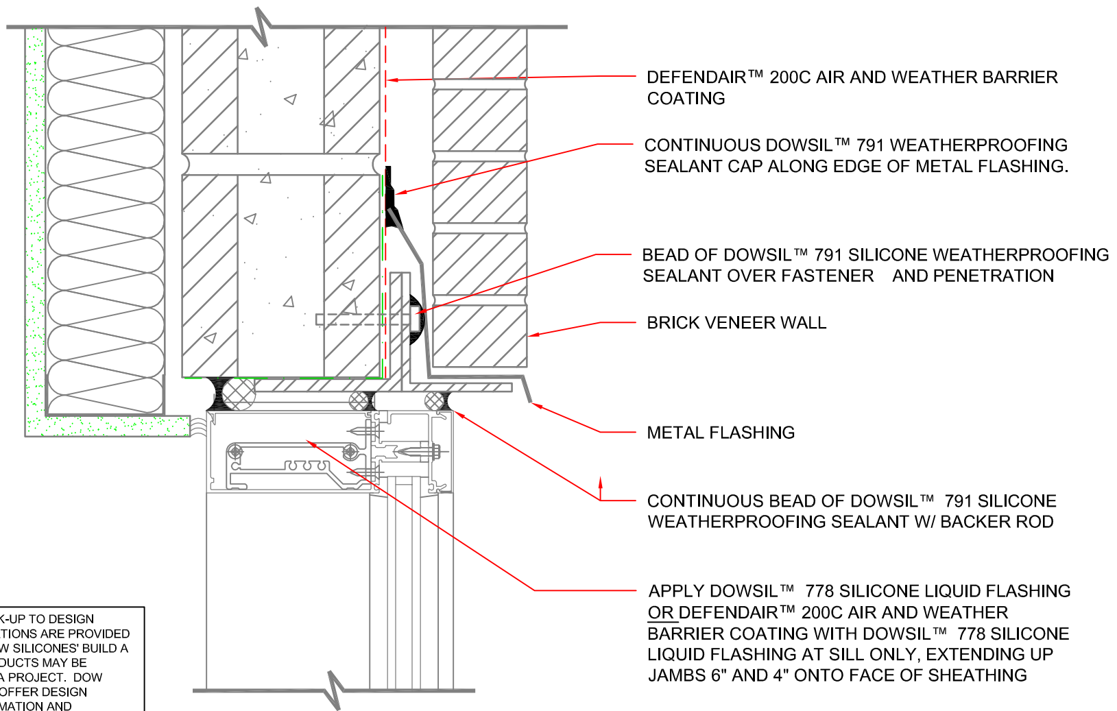
DETAIL SECTION: HEAD : CURTAINWALL AT BRICK W/ CMU WALL SCALE: 3"=1'-0"
