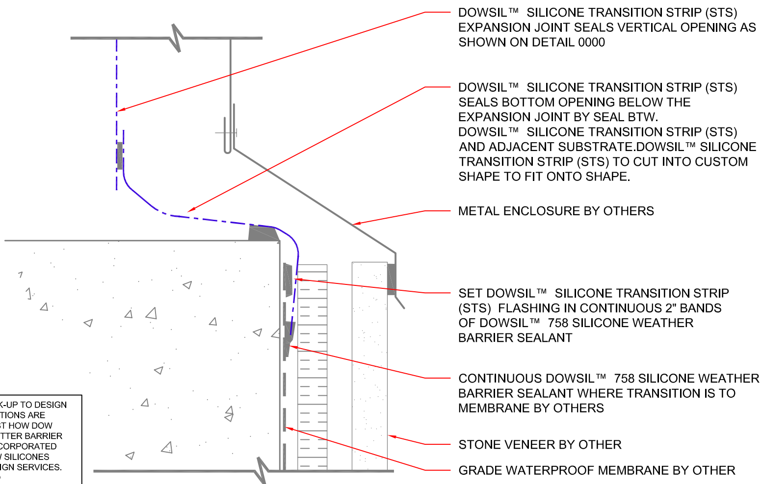
01 DETAIL SECTION: VERTICAL EXPANSION JOINT END SCALE: 3"=1'-0"
