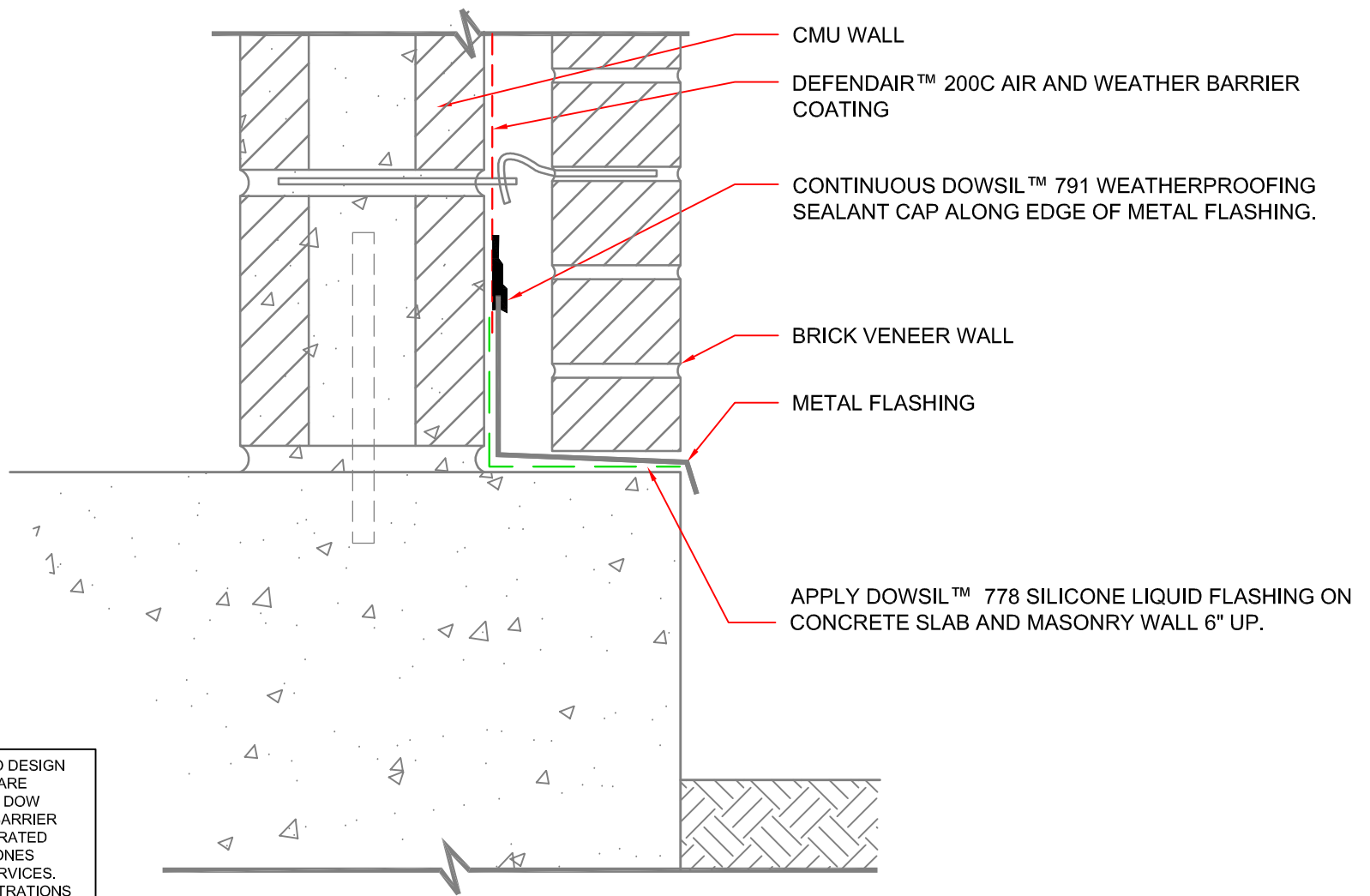
101 DETAIL SECTION: BASE WALL: BRICK W/ CMU WALL SCALE: 3"=1'-0"
