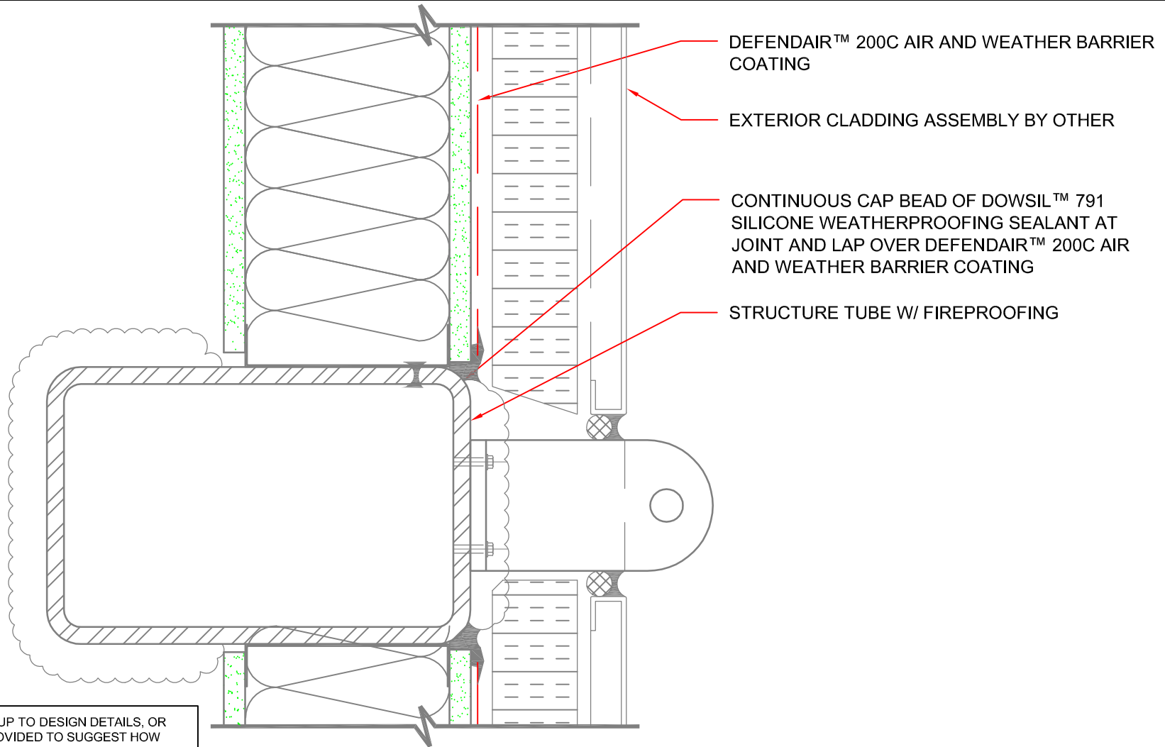
01 DETAIL SECTION: KNIFE PLATE W/ STRUCTURAL STEEL SCALE: 3"=1'-0"
