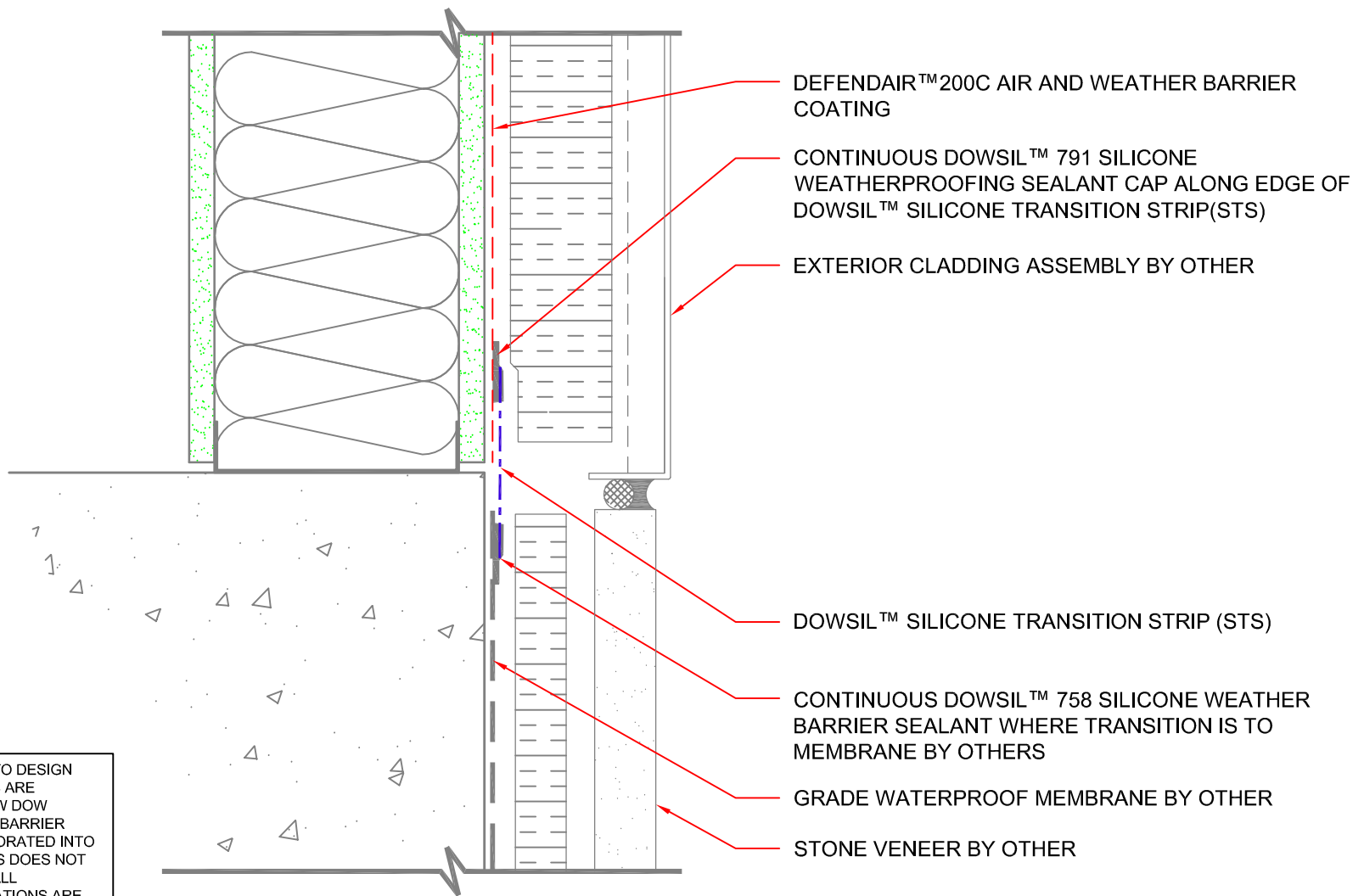
01 ALTERNATE DETAIL SECTION: MTL. STUD WALL TO CONCRETE BASE SCALE: 3"=1'-0"
