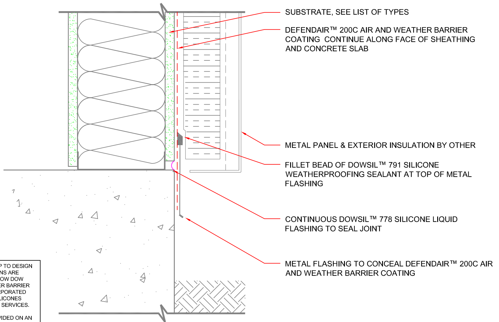
01 ALTERNATE DETAIL SECTION: MTL. STUD WALL TO CONCRETE BASE SCALE: 3"=1'-0"
