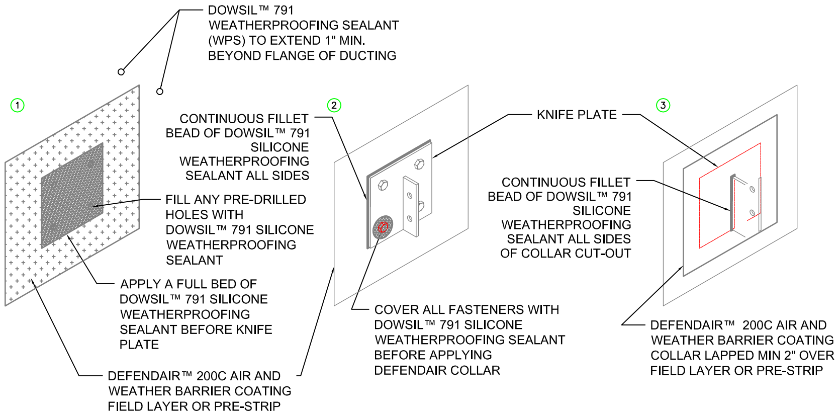
50 FLASHING AT KNIFE PLATE AFTER DEFENDAIR - ISOMETRIC SCALE: N.T.S.
