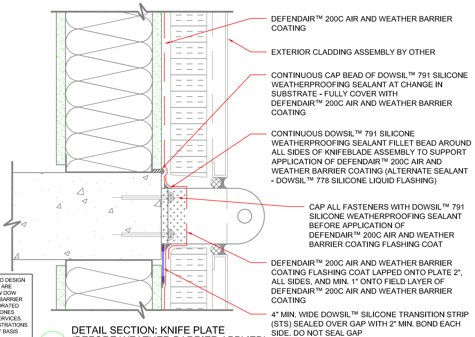
01 DETAIL SECTION: KNIFE PLATE (BEFORE WEATHER BARRIER APPLIED) SCALE: 3"=1'-0"
