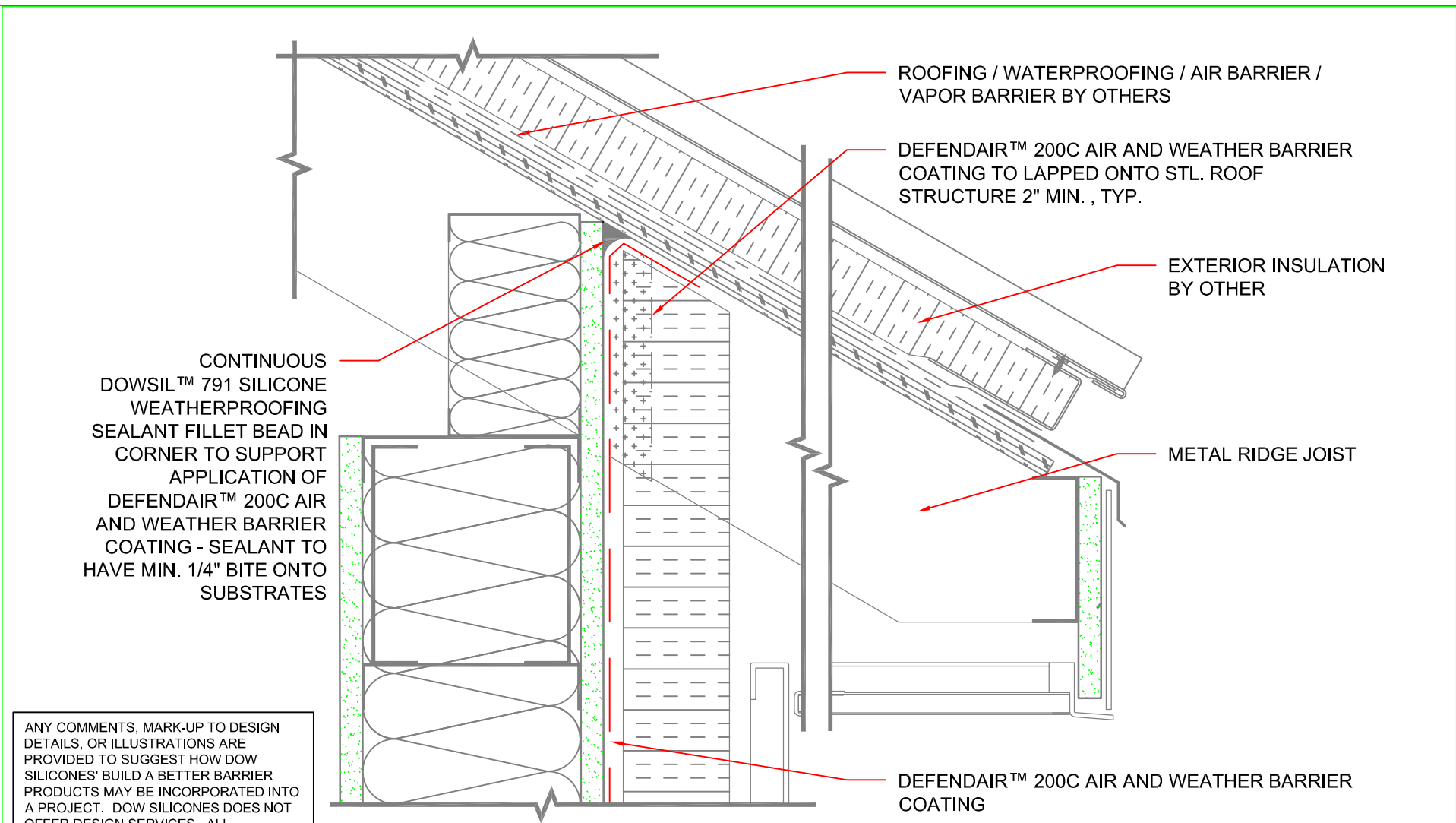
01 DETAIL SECTION: EXTENDED EAVES SCALE: 3"=1'-0"
