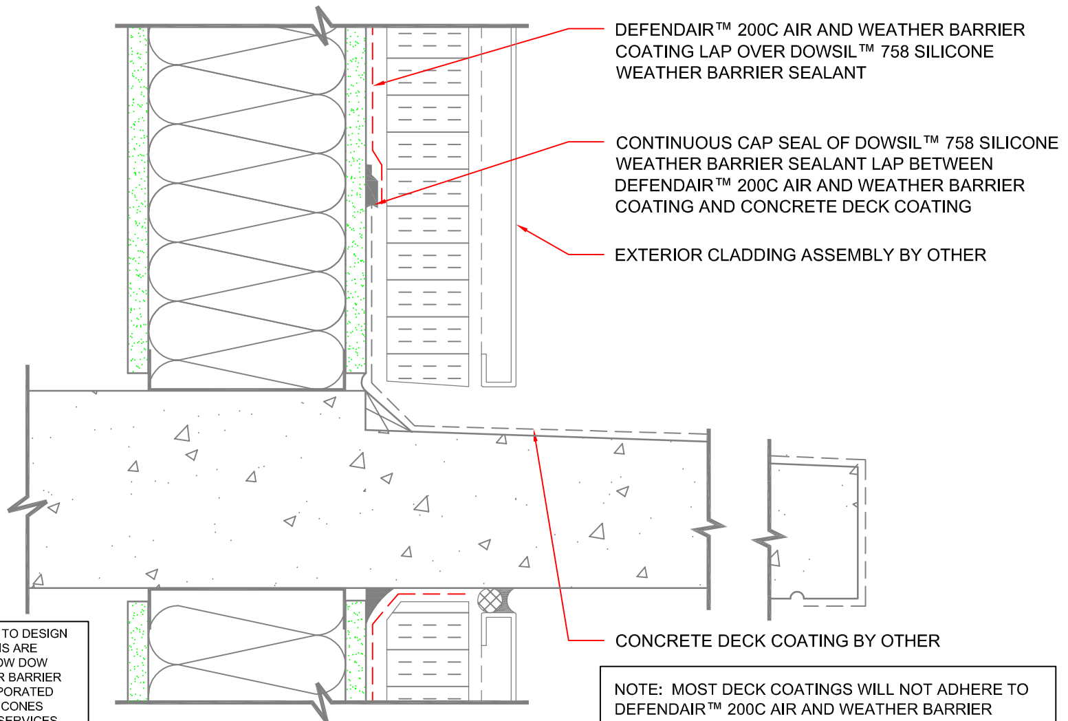
01 DETAIL SECTION: MTL. STUD WALL ON CONG. SLAB SCALE: 3"=1'-0"
