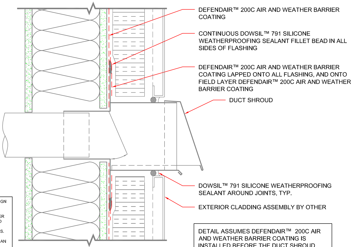
01 DETAIL SECTION: DUCT PENETRATION AT MTL. STUD WALL SCALE: 3"=1'-0"
