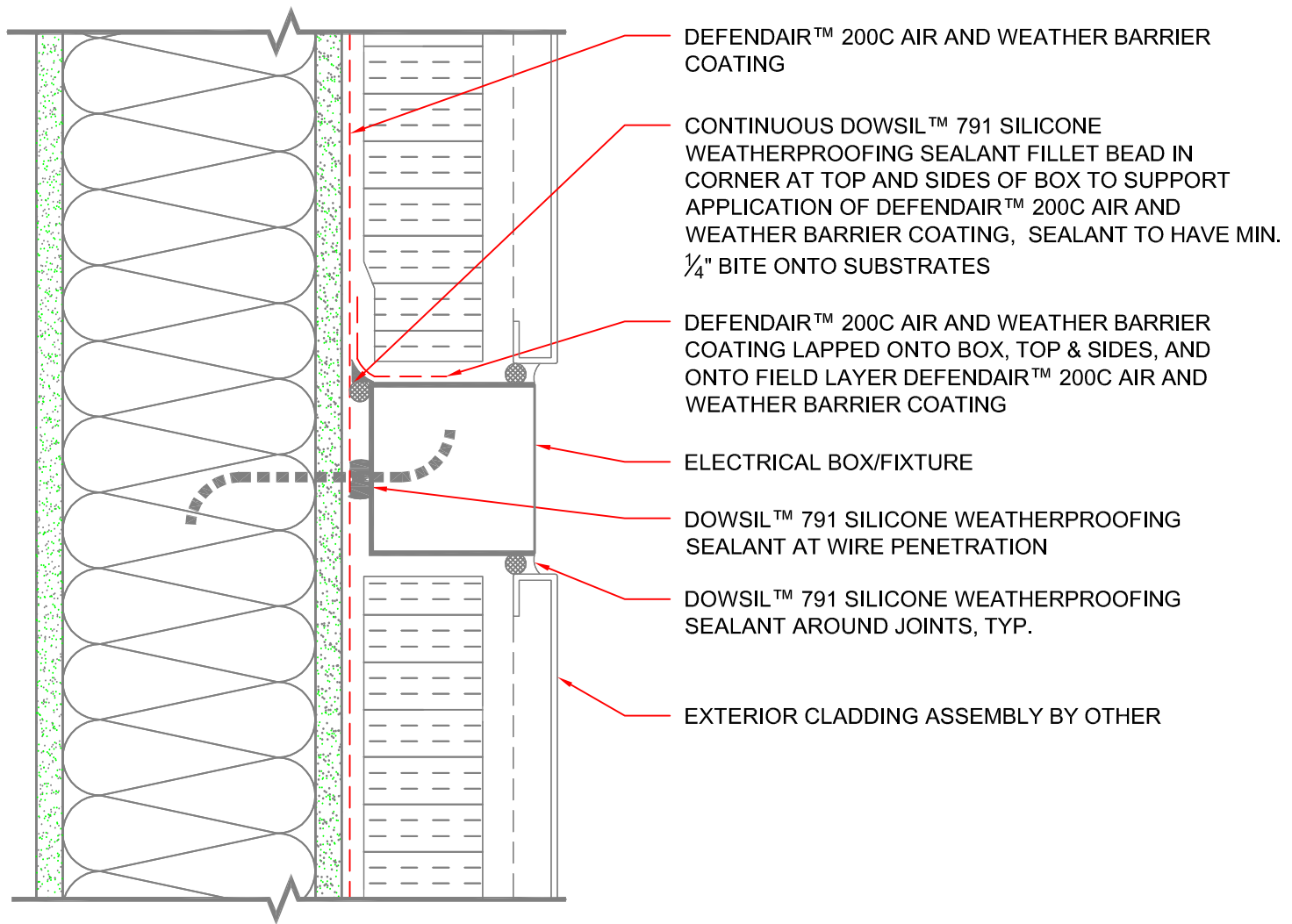
01 DETAIL SECTION: MTL. STUD WALL W/ ELECTRIC BOX SCALE: 3"=1'-0"
