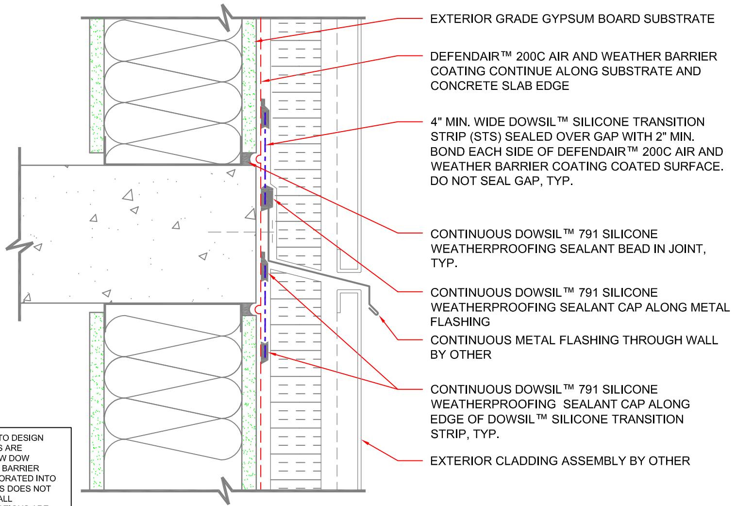
01 DETAIL SECTION: MTL. STUD WALL AT FLOOR SLAB SCALE: 3"=1'-0"
