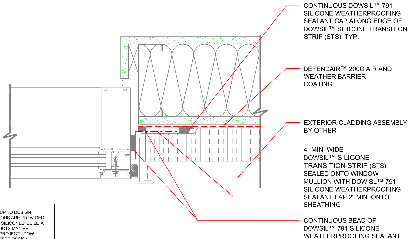
01 DETAIL PLAN: WINDOW JAMB - PROJECTED CURTAIN WALL AT MTL. STUD WALL SCALE: 3"=1'-0"
