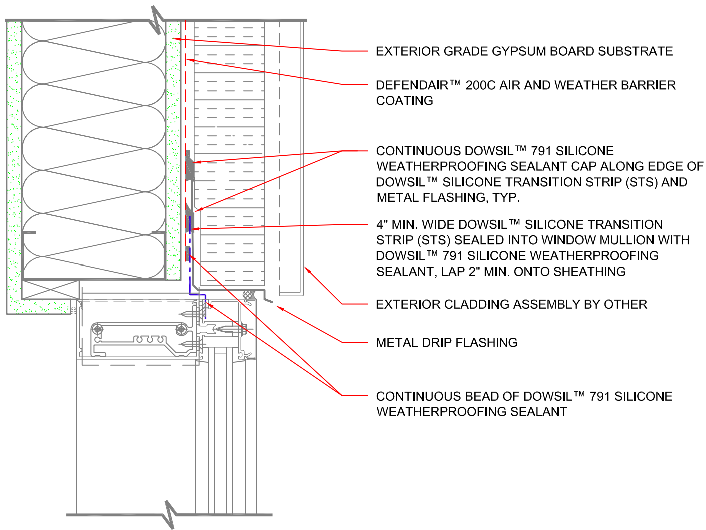
01 DETAIL SECTION: WINDOW HEAD - CURTAIN WALL AT MTL. STUD WALL SCALE: 3"=1'-0"
