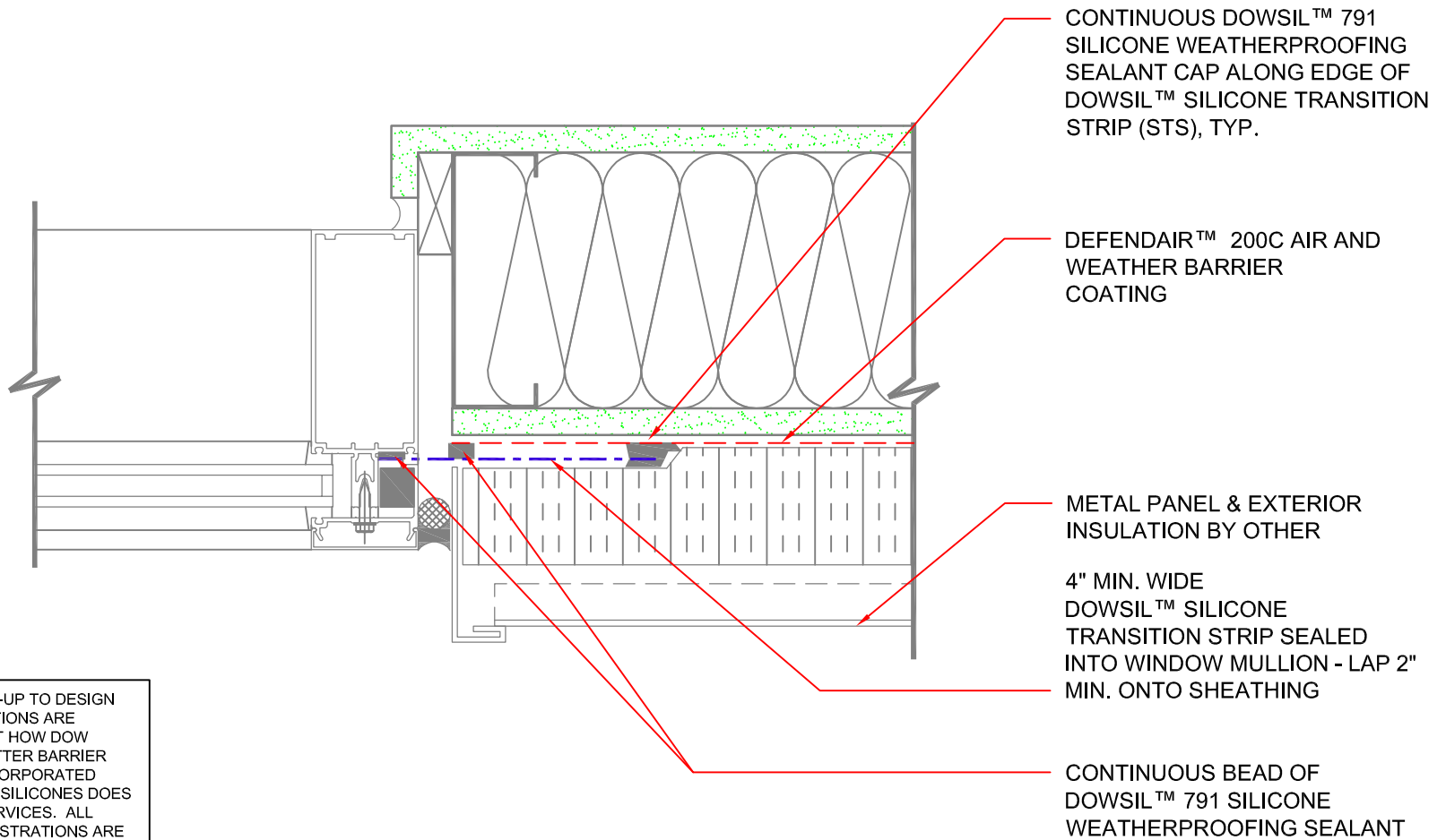
01 DETAIL PLAN: WINDOW JAMB - CURTAINWALL AT MTL. STUD WALL SCALE: 3"=1'-0"
