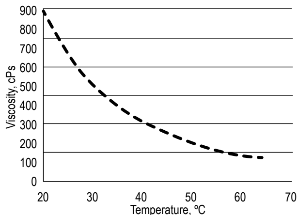
Viscosity versus Temperature DEMTROL™ 2025 Demulsifier
