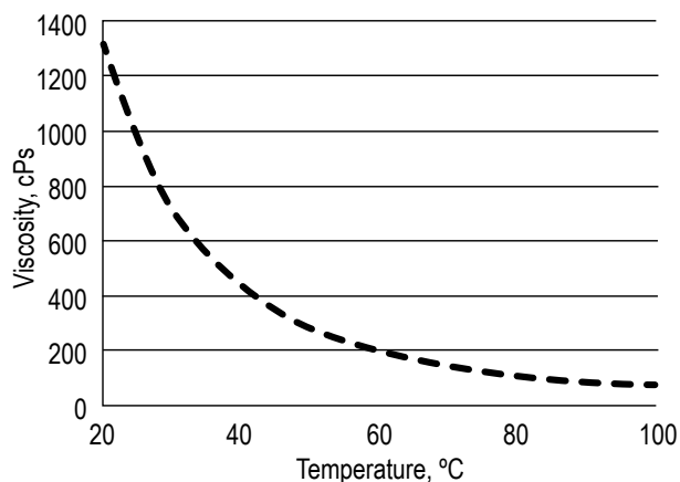
Viscosity versus Temperature DEMTROL™ 1114L Demulsifier
