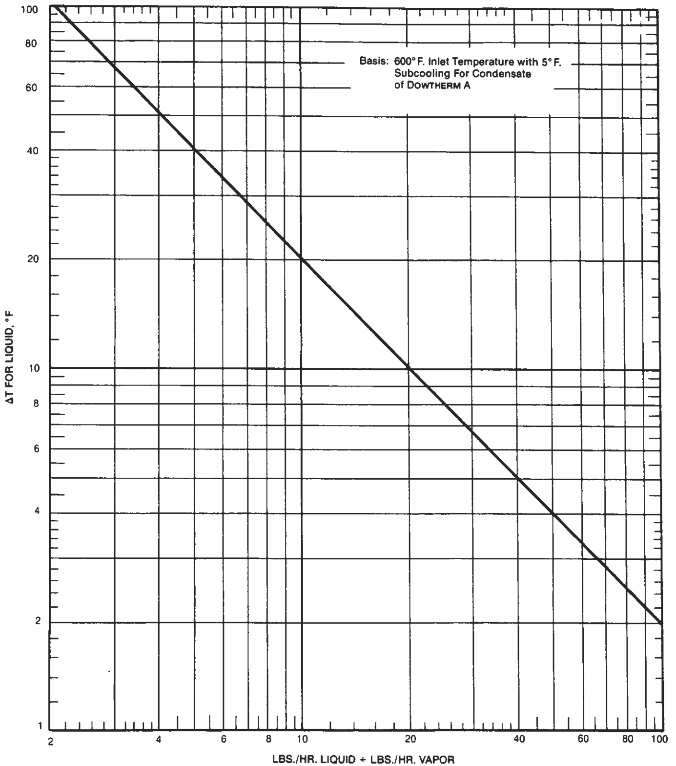
Figure 2 —Comparison of Liquid vs. Vapor Mass Flow Rates for DOWTHERM A Fluid at Various Liquid \Delta T 's
