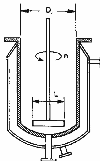
Jacketed Vessels
