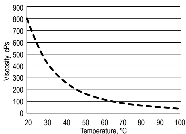
Viscosity versus Temperature DEMTROL™ 1015E Demulsifier
