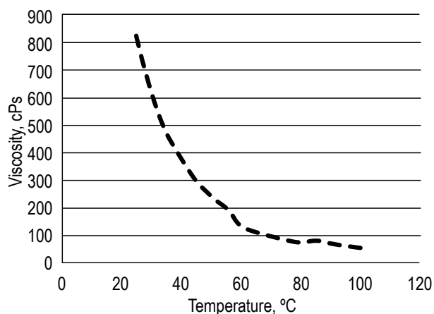
Viscosity versus Temperature DEMTROL™ 4026 Demulsifier
