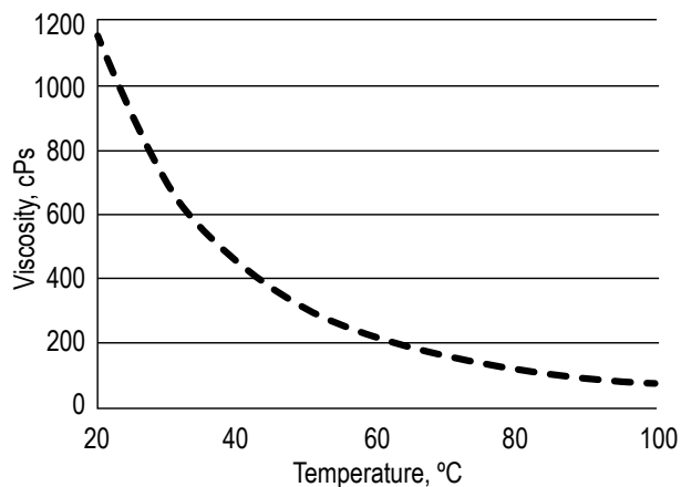
Viscosity versus Temperature DEMTROL™ 2020 Demulsifier
