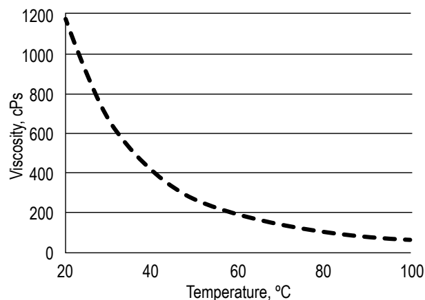
Viscosity versus Temperature DEMTROL™ 1020E Demulsifier
