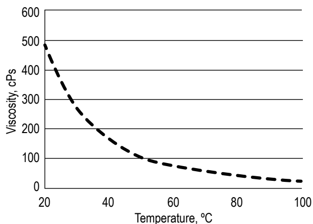
Viscosity versus Temperature DEMTROL™ 1010 Demulsifier
