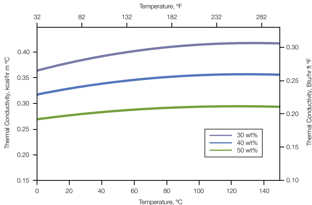
FIGURE 4 • THERMAL CONDUCTIVITY OF UCARSOL™ AP 810 SOLVENT
