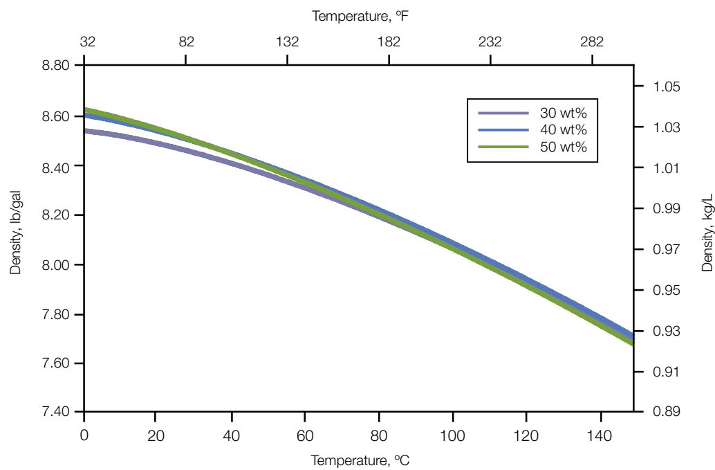
FIGURE 1 • DENSITY OF UCARSOL™ AP 810 SOLVENT
