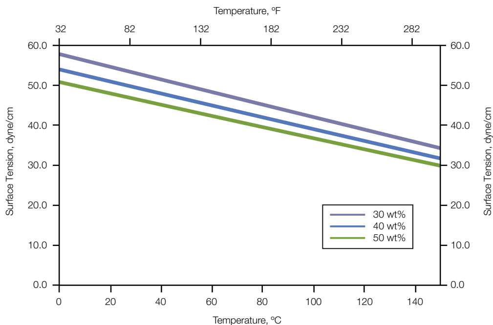
FIGURE 5 • SURFACE TENSION OF UCARSOL™ AP 810 SOLVENT
