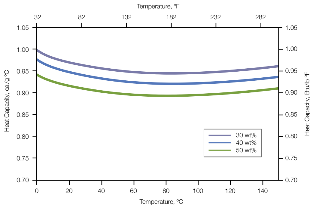
FIGURE 3 • HEAT CAPACITY OF UCARSOL™ AP 810 SOLVENT
