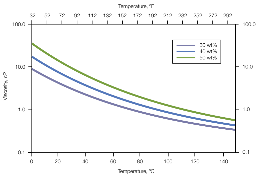
FIGURE 2 • VISCOSITY OF UCARSOL™ AP 810 SOLVENT
