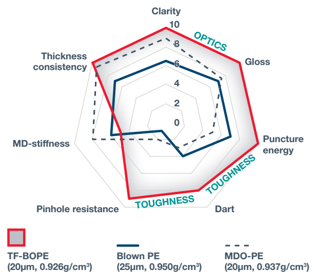
Figure 1: TF-BOPE film vs. other PE films
