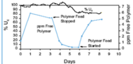
FIGURE 3a. POLYMER UNDERFEEDING DISCOVERED TOO LATE (OPTIDOSE 2000/ALL-ORGANIC PROGRAM)
