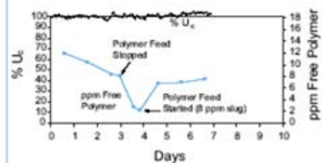
FIGURE 2b. POLYMER UNDERFEEDING DISCOVERED BEFORE FOULING OCCURS (OPTIDOSE 3100/STABILIZED PHOSPHATE PROGRAM)
