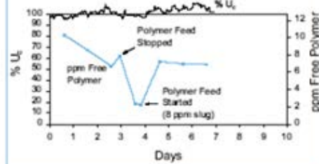
FIGURE 2b. POLYMER UNDERFEEDING DISCOVERED BEFORE FOULING OCCURS (OPTIDOSE 3100/STABILIZED PHOSPHATE PROGRAM)
