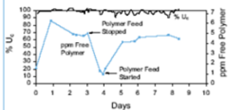
FIGURE 3b. POLYMER UNDERFEEDING DISCOVERED BEFORE FOULING OCCURS (OPTIDOSE 2000/ALL-ORGANIC PROGRAM)
