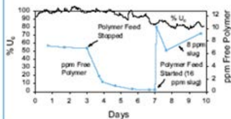
FIGURE 2a. POLYMER UNDERFEEDING DISCOVERED TOO LATE (OPTIDOSE 3100/STABILIZED PHOSPHATE PROGRAM)
