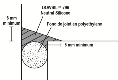
Figure 3: Joint d'angle.
