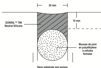
Figure 1: Joint profond.
