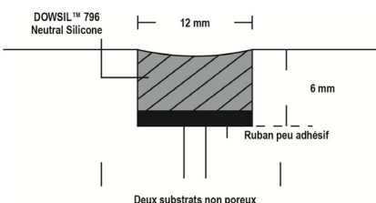
Figure 2: Joint étroit.
