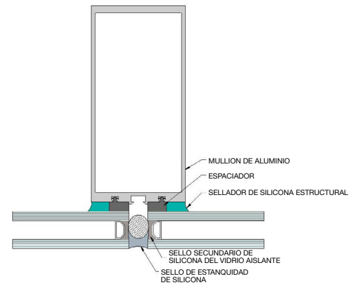
MULLION VERTICAL
