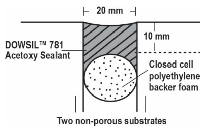
Figure 1: Joint profonde
