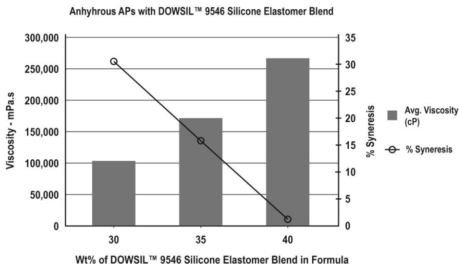
Figure 6: In soft solid applications, DOWSIL™ 9546 Silicone Elastomer Blend significantly reduces syneresis.
