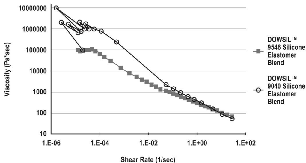
Figure 2: Rheological flow comparison of DOWSIL™ 9546 Silicone Elastomer Blend and DOWSIL™ 9040 Silicone Elastomer Blend.
