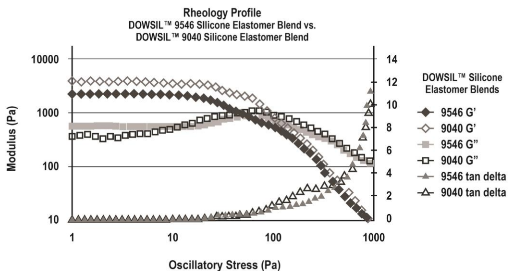
Figure 3: Rheology profile comparison of DOWSIL™ 9546 Silicone Elastomer Blend and DOWSIL™ 9040 Silicone Elastomer Blend.
