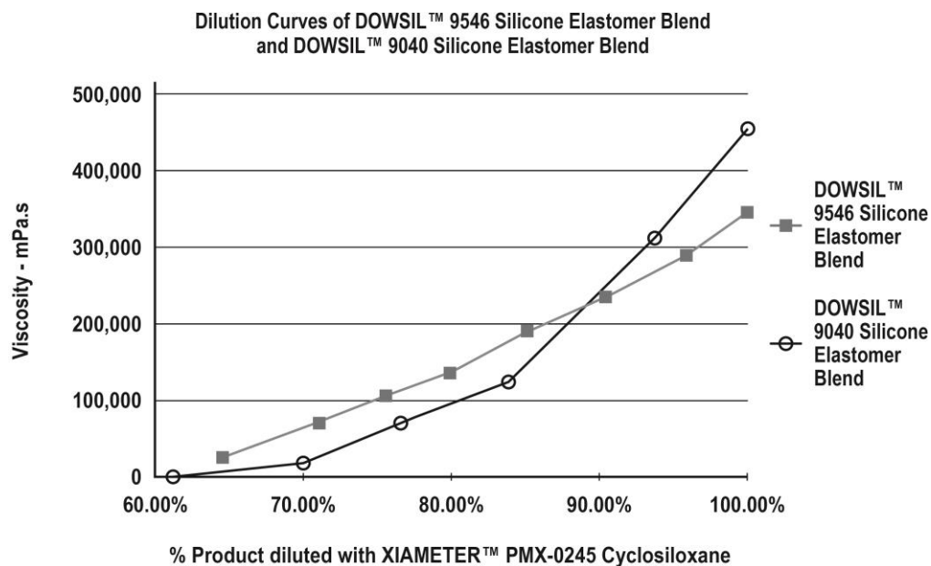
Figure 1: Dilution curves comparing DOWSIL™ 9546 Silicone Elastomer Blend and DOWSIL™ 9040 Silicone Elastomer Blend.
