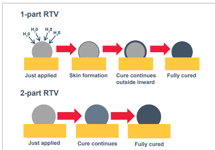
Figure 1. Cure mechanism of condensation 1-part versus 2-part RTV adhesives
