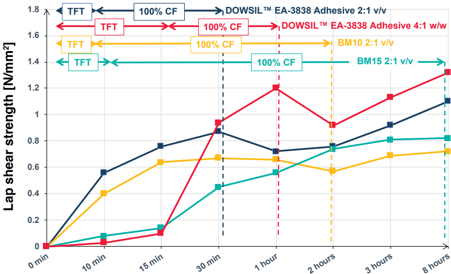
Figure 2. Time-dependent, early lap shear adhesion development after assembly of a stainless steel joint bonded on glass
