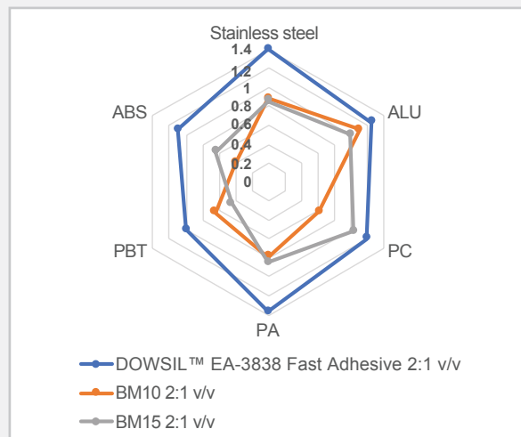
Figure 3. Lap shear strength [N/mm²] after one week for different substrates, alongside different applications/markets requiring fast and robust adhesion to metals, plastics, ceramics, and composites (including renewables, EV charging stations, display bonding, power electronics, appliances, and many more)
