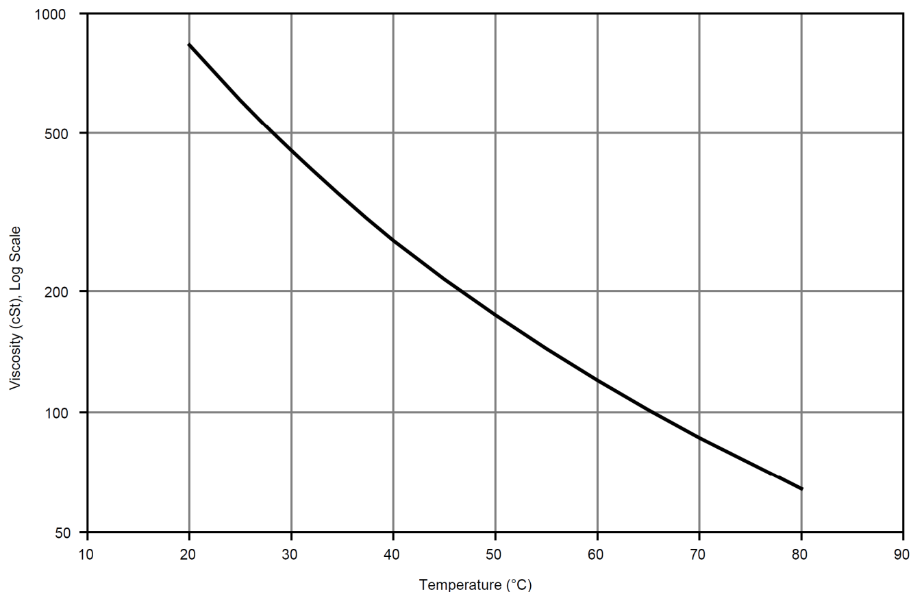
Figure 1: Viscosity (Kinematic) vs. Temperature
