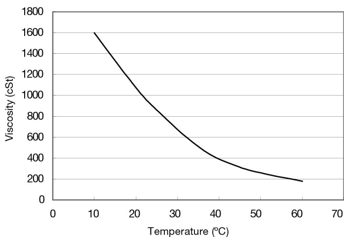
Figure 1: Viscosity vs. Temperature
