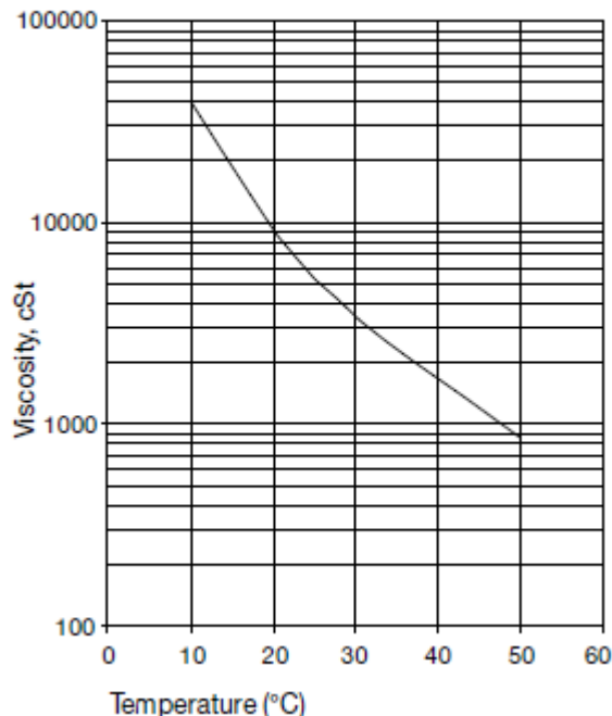
Viscosity vs. Temperature of VORANOL RN 411
