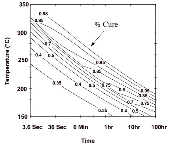
Figure 5. BCB % cure vs time and temperature
