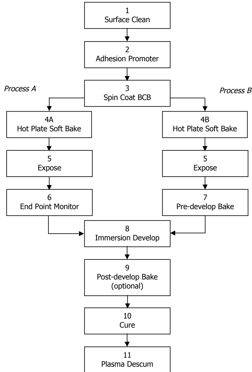
Figure 2. Process Flows for CYCLOTENE 4000 Series Advanced Electronic Resins
